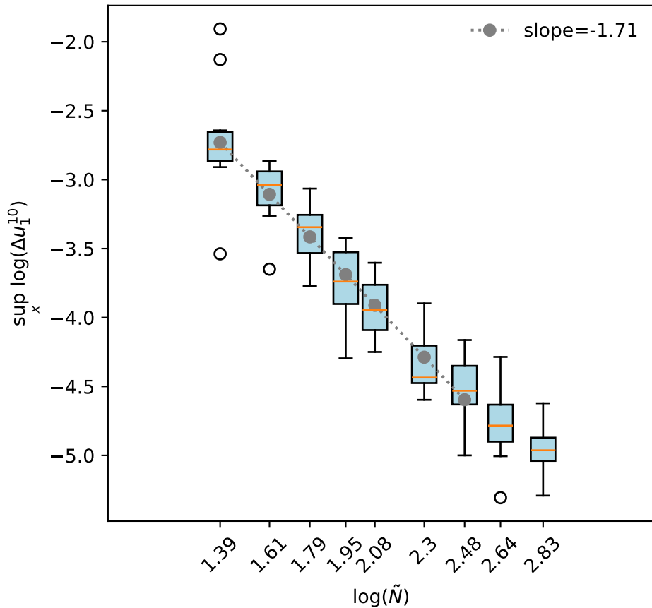
Max log-errors in u(x) v/s \log(\tilde{N})
