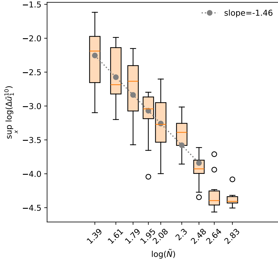
Max log-errors in \bar{u}(x) v/s \log(\tilde{N})
