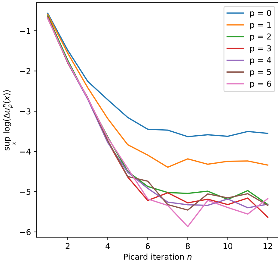
Max log error in u(x) vs Picard iterations
