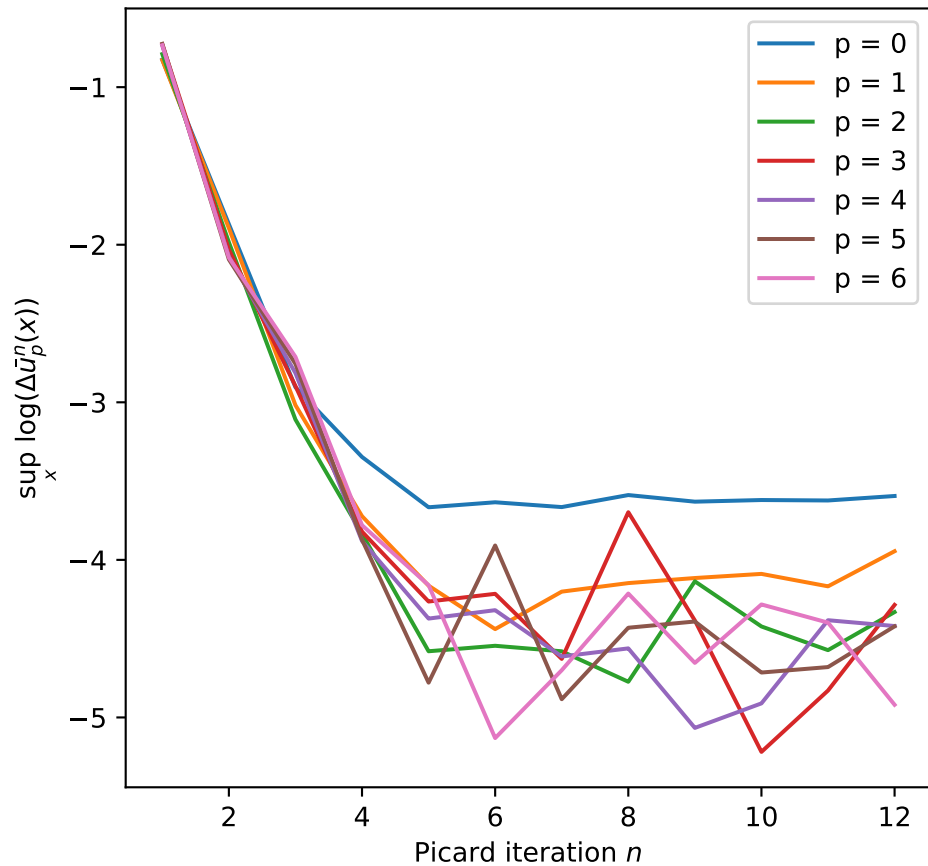
Max log error in \bar{u}(x) vs Picard iterations
