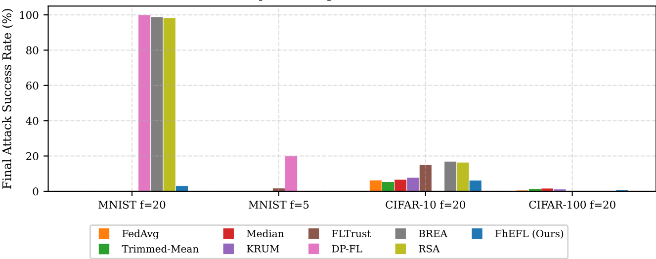
Final ASR Comparison (avg. last 10 rounds) [lower is better]
