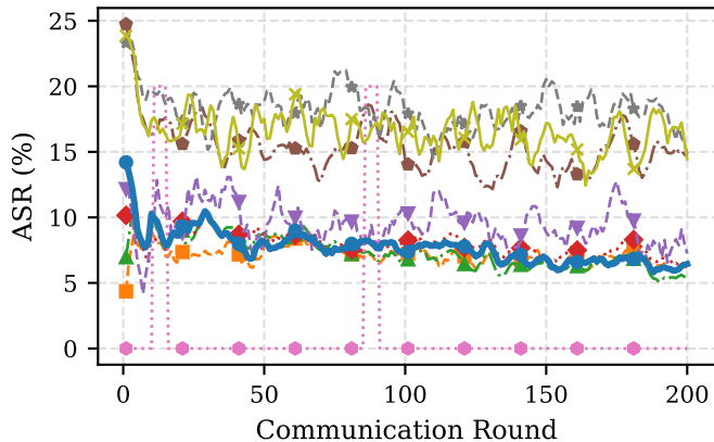
Attack Success Rate — CIFAR-10 (f=20)
