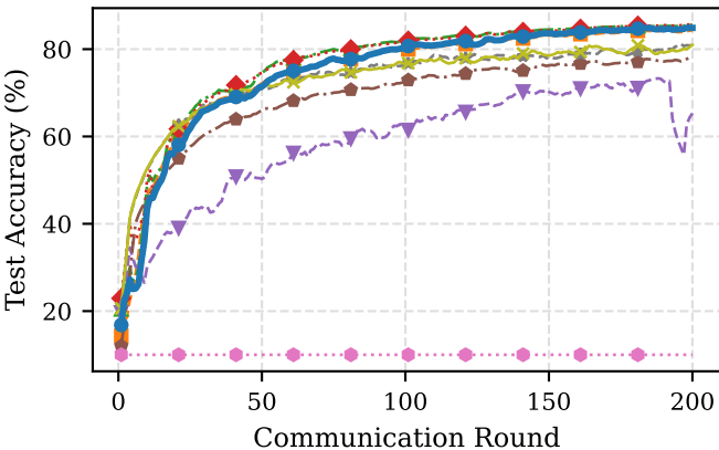
Test Accuracy — CIFAR-10 (f=20)
