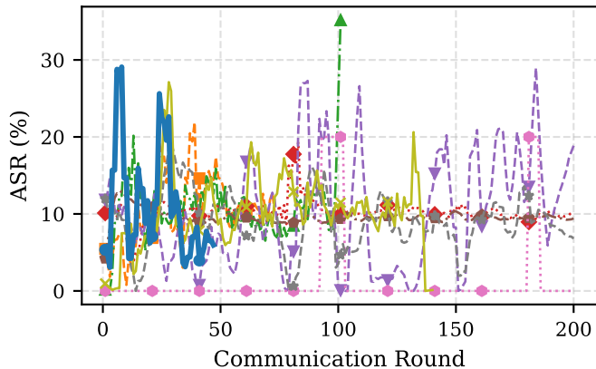
ASR — Model Poisoning CIFAR-10 (f=20)
