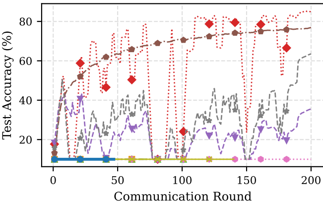
Test Accuracy — Model Poisoning CIFAR-10 (f=20)
