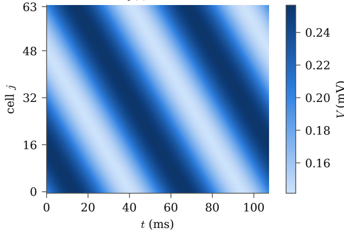
(b) N=64 : V_j(t) over two periods
