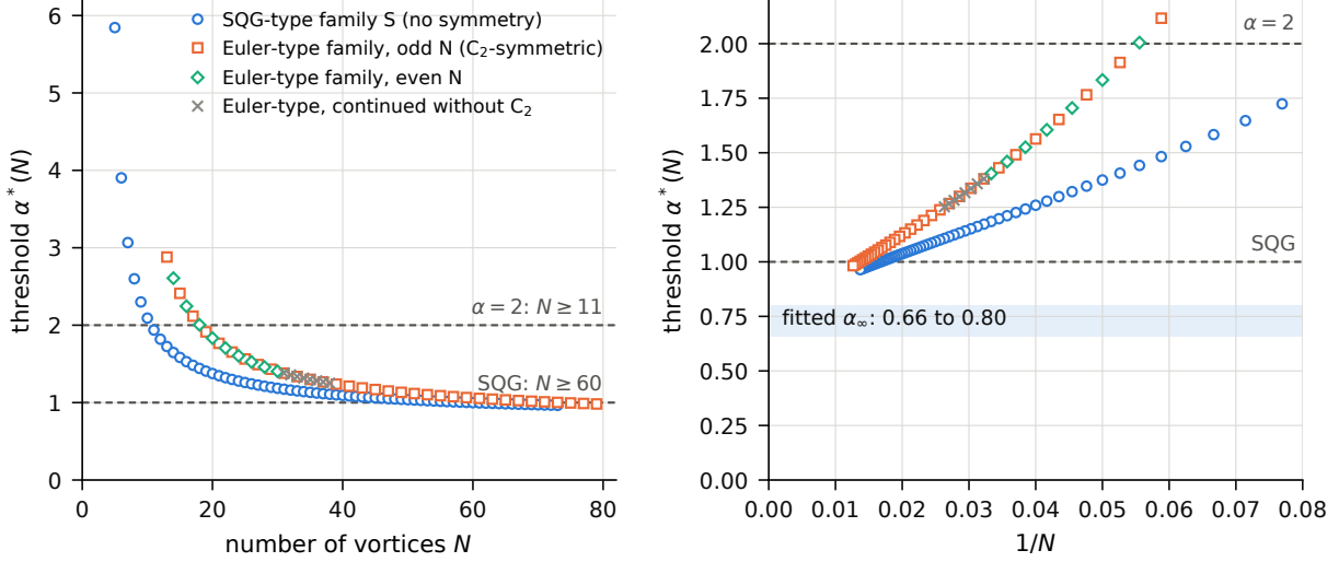
Figure 1: The least \alpha at which N vortices collapse self-similarly without rotation, along four families (numerical). Left: against N ; the dashed lines are \alpha = 2 and SQG ( \alpha = 1 ), crossed by the SQG-type family at N = 11 and N = 60 . Right: against 1/N ; the band is the range 0.66 to 0.80 of the limits \alpha_\infty given by the fits of Table 3. The data are in data/phase-diagram/alpha-star-phase-diagram.csv .
