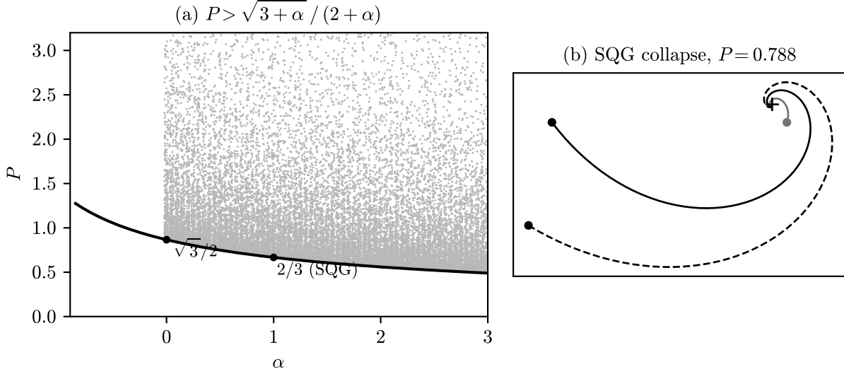
Figure 3: (a) The bound B(\alpha) of Theorem 2 (curve) and P = |S|/(8A) , in double precision, for 24395 random collapsing triangles at 61 values of \alpha from 0 to 3, with the shortest side between 10^{-3} and 1 times the middle one (dots, spread slightly in \alpha for visibility); none lies below the curve, which is drawn from \alpha = -0.85 and approached as the shortest side tends to 0. (b) The paths of the three vortices of an SQG collapse ( \alpha = 1 ) with sides 0.45 , 1 and (1 + 0.45m_*)^{1/2} and the circulations of Lemma 5, integrated from (1) to 10^{-6}t_c before the collapse; dots mark the initial positions and the cross the collision point. The program is plot_alpha_winding.py .
