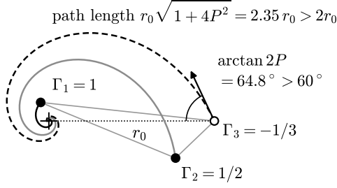
Figure 2: Minimizing configurations on \mathcal{A}_- (dots, filled for positive circulation) and the logarithmic spiral paths of their vortices into the collision point (+), drawn until the distances have shrunk by the factor 100, for (a) \mu = 1/2 and (b) \mu = 0.05 , where the two weak vortices form a tight pair beside the strong one, as in Theorem 3, and P is close to \sqrt{3}/2 . Each path meets the line to the collision point at the constant angle \arctan 2P > 60^\circ and has length r_0\sqrt{1+4P^2} > 2r_0 (Corollary 1), marked here for the third vortex.
