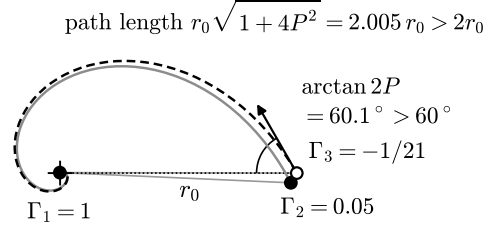
Figure 2: Minimizing configurations on \mathcal{A}_- (dots, filled for positive circulation) and the logarithmic spiral paths of their vortices into the collision point (+), drawn until the distances have shrunk by the factor 100, for (a) \mu = 1/2 and (b) \mu = 0.05 , where the two weak vortices form a tight pair beside the strong one, as in Theorem 3, and P is close to \sqrt{3}/2 . Each path meets the line to the collision point at the constant angle \arctan 2P > 60^\circ and has length r_0\sqrt{1+4P^2} > 2r_0 (Corollary 1), marked here for the third vortex.
