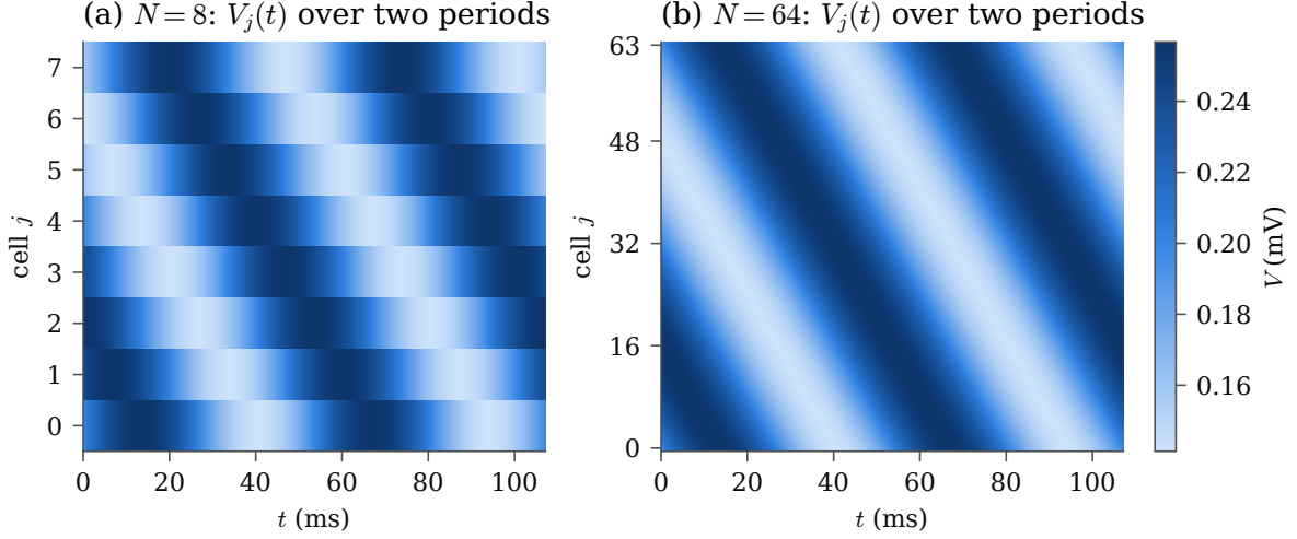
Figure 2: The rotating 1-wave of Theorem B on rings of (a) N = 8 and (b) N = 64 cells: V_j(t) = \phi_{*,V}(\omega_*t + 2\pi j/N) , one row per cell j , over two periods, 0 \leq t \leq 2T , with one color scale for both panels. The profile is the V component of the center of the existence proof for that N (code/fourier/data/centre_N8_K32.json and centre_N64_K32.json, hashed by data/fourier-existence-N8.json and -N64.json), summed in binary64 at 600 times per row, with the frequency \bar{\omega} of the center in place of \omega_* ; by Theorem B(a) the profile of the wave differs from it by at most r_{\text{ex}}/4 mV and |\omega_* - \bar{\omega}| \leq r_{\text{ex}} (Table 1). Since x_j(t) = x_0(t + jT/N) , each cell runs T/N ahead of cell j - 1 , and the crests move toward decreasing j , once around the ring in each period. The periods are not drawn as data; Theorem B(b) encloses them in [53.58797097681944967415082, 53.58797097681944967415083] ms for N = 8 and [53.58810041831757754104213, 53.58810041831757754104214] ms for N = 64 . The figure shows the wave only, not its stability (Theorem B(c)). Reproduced by code/plot_cardiac_rings.py.
