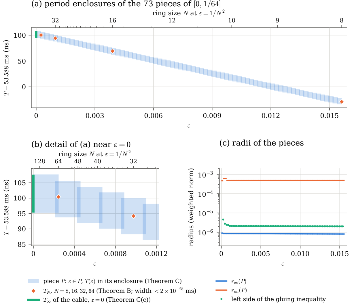
Figure 3: The pieces of the proof of Theorem C, as stored in data/fourier-existence-alln.json . (a) Each of the 73 boxes is a piece P (width 1/4096 ; consecutive pieces overlap by 1/32768 and are darker where they overlap) times its period interval: for every \varepsilon \in P , T(\varepsilon) = 2\pi/\omega_*(\varepsilon) lies in that interval. Diamonds: the periods T_N of Theorem B at \varepsilon = 1/N^2 , N = 8, 16, 32, 64 (Table 1), whose enclosures are narrower than 2 \times 10^{-25} ms; each lies in the period interval of every piece that contains 1/N^2 (Table 3). Bar at \varepsilon = 0 : the period T_\infty \in [53.58809529823299300232974, 53.58810763684487454838746] ms of the cable wave (Theorem C(c)), the interval of the piece [0, 1/4096] . The vertical axis is T - 53.588 ms in ns; 53.588 ms is an axis offset, not a result. The top axes mark \varepsilon = 1/N^2 at the labelled N , with minor ticks at the other integers N up to 29 in (a) and up to 52 in (b); these points accumulate at \varepsilon = 0 . (b) The part of (a) with \varepsilon \leq 5/4096 : the rings N = 32 and N = 64 ( 1/4096 lies in two pieces) and the cable. (c) For each piece, the existence radius r_{\text{ex}}(P) and the uniqueness radius r_{\text{un}}(P) , drawn over the piece, both in the weighted norm \|\cdot\|_\eta of that piece; and, at the middle of each of the 72 overlaps, the left side of the gluing inequality (10), in the norm of the later piece P_b , which must not exceed r_{\text{un}}(b) ; its largest ratio to r_{\text{un}}(b) is below 0.0076 (Section 4.8). The weights differ from piece to piece, so the values in (c) are not in one common norm. The figure draws stored enclosures and radii only; stability is proved only for N = 8, 16, 32, 64 . Reproduced by code/plot_cardiac_rings.py .
