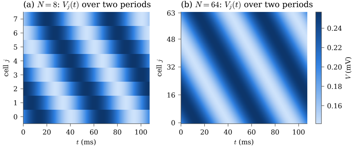
Figure 2: The rotating 1-wave of Theorem B on rings of (a) N = 8 and (b) N = 64 cells: V_j(t) = \phi_{*,V}(\omega_*t + 2\pi j/N) , one row per cell j , over two periods, 0 \leq t \leq 2T , with one color scale for both panels. The profile is the V component of the center of the existence proof for that N (code/fourier/data/centre_N8_K32.json and centre_N64_K32.json, hashed by data/fourier-existence-N8.json and -N64.json), summed in binary64 at 600 times per row, with the frequency \bar{\omega} of the center in place of \omega_* ; by Theorem B(a) the profile of the wave differs from it by at most r_{\text{ex}}/4 mV and |\omega_* - \bar{\omega}| \leq r_{\text{ex}} (Table 1). Since x_j(t) = x_0(t + jT/N) , each cell runs T/N ahead of cell j - 1 , and the crests move toward decreasing j , once around the ring in each period. The periods are not drawn as data; Theorem B(b) encloses them in [53.58797097681944967415082, 53.58797097681944967415083] ms for N = 8 and [53.58810041831757754104213, 53.58810041831757754104214] ms for N = 64 . The figure shows the wave only, not its stability (Theorem B(c)). Reproduced by code/plot_cardiac_rings.py.
