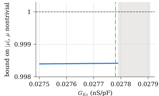
(c) Floquet multiplier bound
