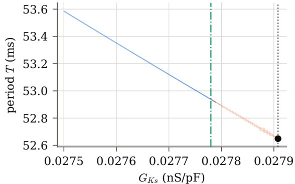
(c) Floquet multiplier bound
