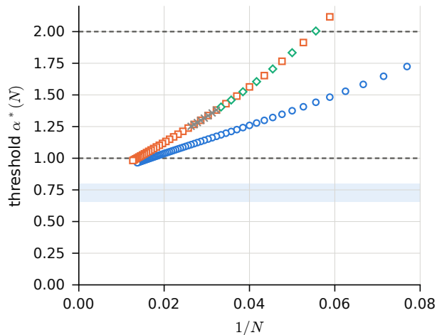
(b) Reciprocal vortex count
