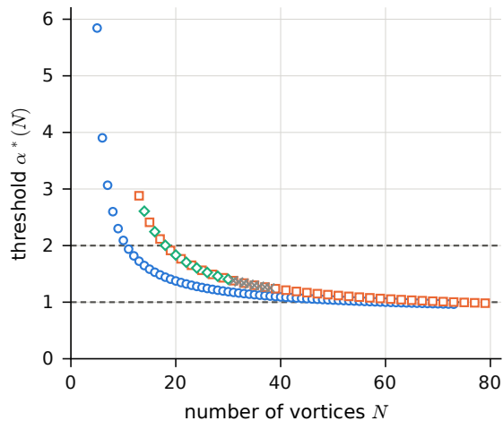
(a) Finite vortex counts
