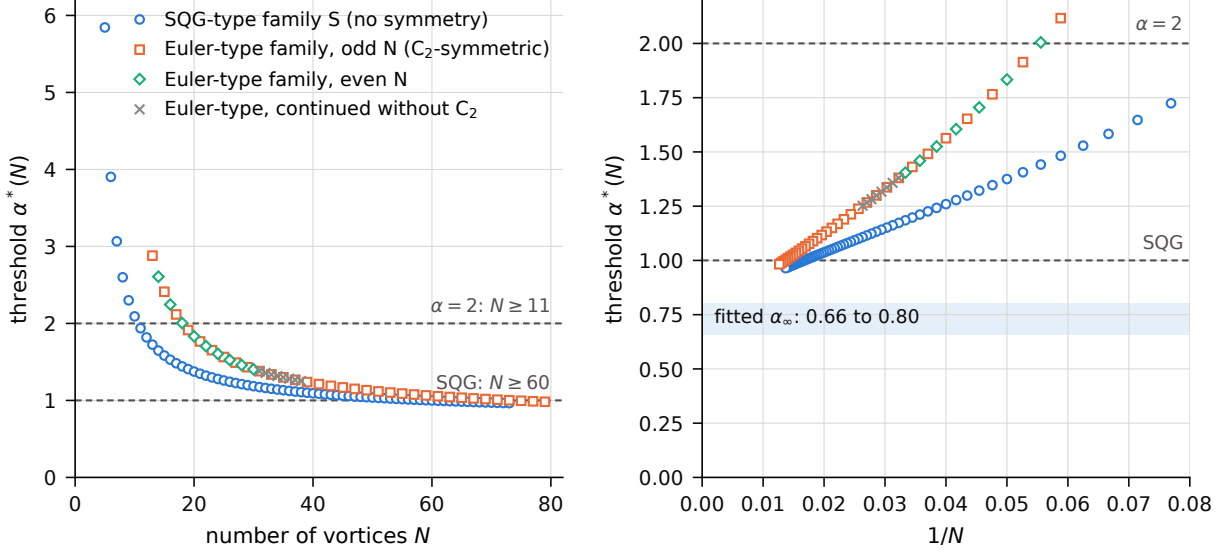
Figure 1: The least \alpha at which N vortices collapse self-similarly without rotation, along the two families S and E below, with the odd, even and asymmetric branches of E drawn separately (numerical). Left: against N ; the dashed lines are \alpha = 2 and SQG ( \alpha = 1 ), crossed by the SQG-type family at N = 11 and N = 60 . Right: against 1/N ; the band is the range 0.66 to 0.80 of the limits \alpha_\infty given by the fits of Table 3. All axes are dimensionless. The band summarizes a range of extrapolation fits, not a confidence interval. The data are in data/phase-diagram/alpha-star-phase-diagram.csv ; plot_phase_diagram.py reads these data and the stored fit ranges to reproduce the figure.
