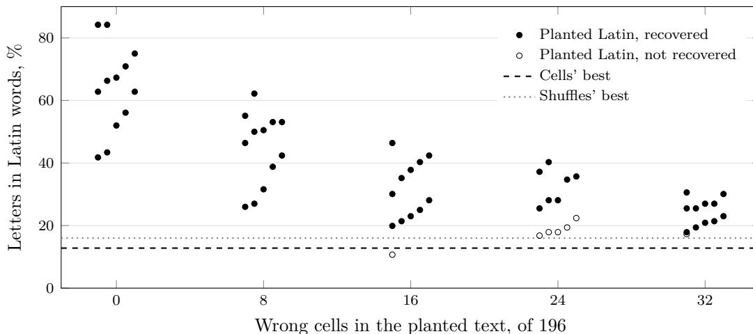
Figure 3: Share of letters in Latin words of five letters or more, for the 60 planted Latin texts by the number of wrong cells given to them, each decrypted with the key its search found; filled marks are texts recovered with at least 90 percent of clean cells right, open marks the rest, and marks are spread a little sideways so none hides another. The dashed line is the cells’ best over 41 searches and the dotted line the best of the 4 shuffles searched the same way.
