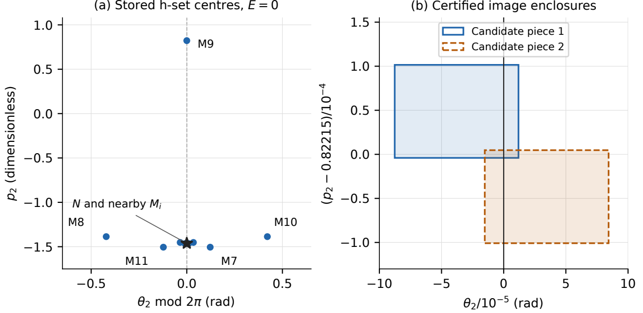
Figure 1: The section geometry at E = 0 , in the dimensionless units m = l = g = 1 . (a) Centres of the 23 configured h-sets in horseshoe_E0.cfg , with angles reduced modulo 2\pi ; the star marks the centre of N . These are numerical design points, not a trajectory or a rendering of the invariant manifolds; the small h-set widths are not resolved at this scale. (b) The two rectangular image enclosures printed in data/E0.txt for the candidate pieces that may meet the symmetry line \theta_2 = 0 . Coordinates are rescaled to resolve the certified bounds near q_0 ; overlapping rectangles do not mean that the actual images overlap. The boxes contain images of pieces of the search strip, not just the homoclinic point. Transversality follows from the certified tangent-slope bounds and the lemmas, not from the plotted rectangles. No new integration is used in either panel.
