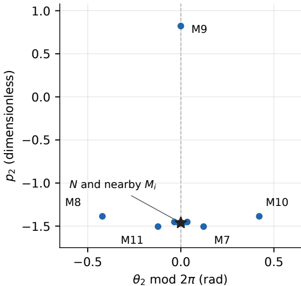
(a) Stored h-set centres, E = 0
