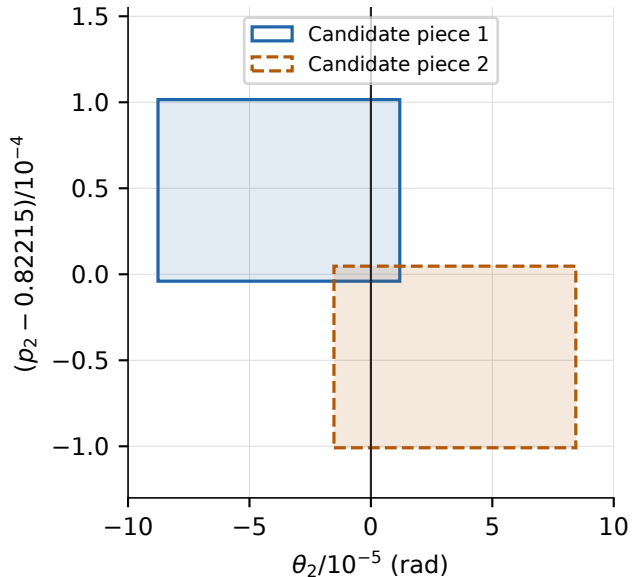
(b) Certified image enclosures
