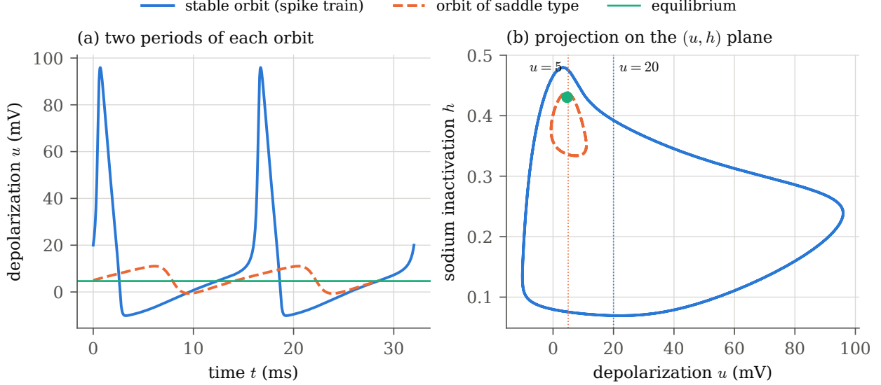
Figure 2: The orbits of Theorem 5 at J = 8 , E_l = 10.613 , integrated in floating point from the high-precision section points of Section 8 ( code/hh_make_figures.py ). (a) u(t) over two periods of the stable orbit \Gamma_s (solid) and of the saddle-type orbit \Gamma_u (dashed), and the equilibrium u^* . (b) The projection on the (u, h) plane, with the sections u = 20 and u = 5 (dotted) and the equilibrium (dot). The enclosures of the theorems are far narrower than the lines.
