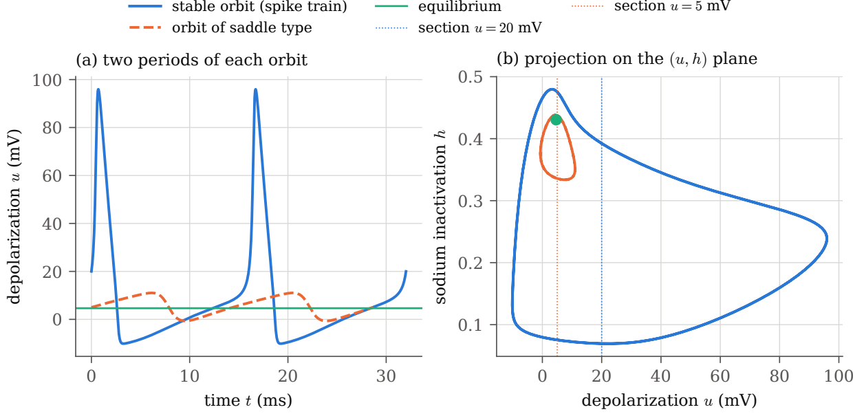
Figure 2: The orbits of Theorem 5 at J = 8 , E_l = 10.613 , integrated in floating point from the high-precision section points of Section 8 (code/hh_make_figures.py). (a) u(t) over two periods of the stable orbit \Gamma_s (solid) and of the saddle-type orbit \Gamma_u (dashed), and the equilibrium u^* . (b) The projection on the (u, h) plane, with the sections u = 20 and u = 5 (dotted) and the equilibrium (dot). The enclosures of the theorems are far narrower than the lines.
