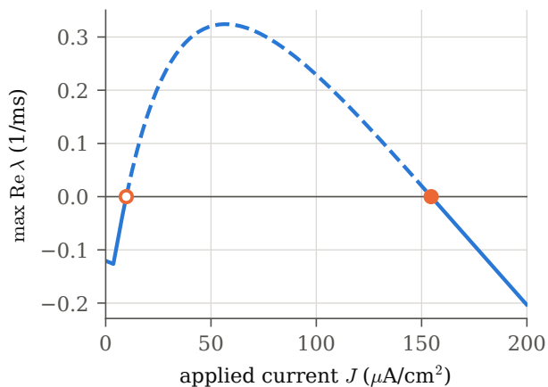
(b) the leading eigenvalues
