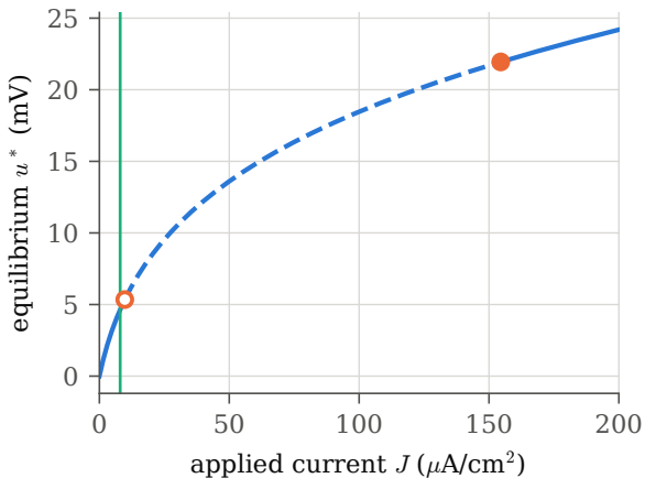
(a) the branch of equilibria
