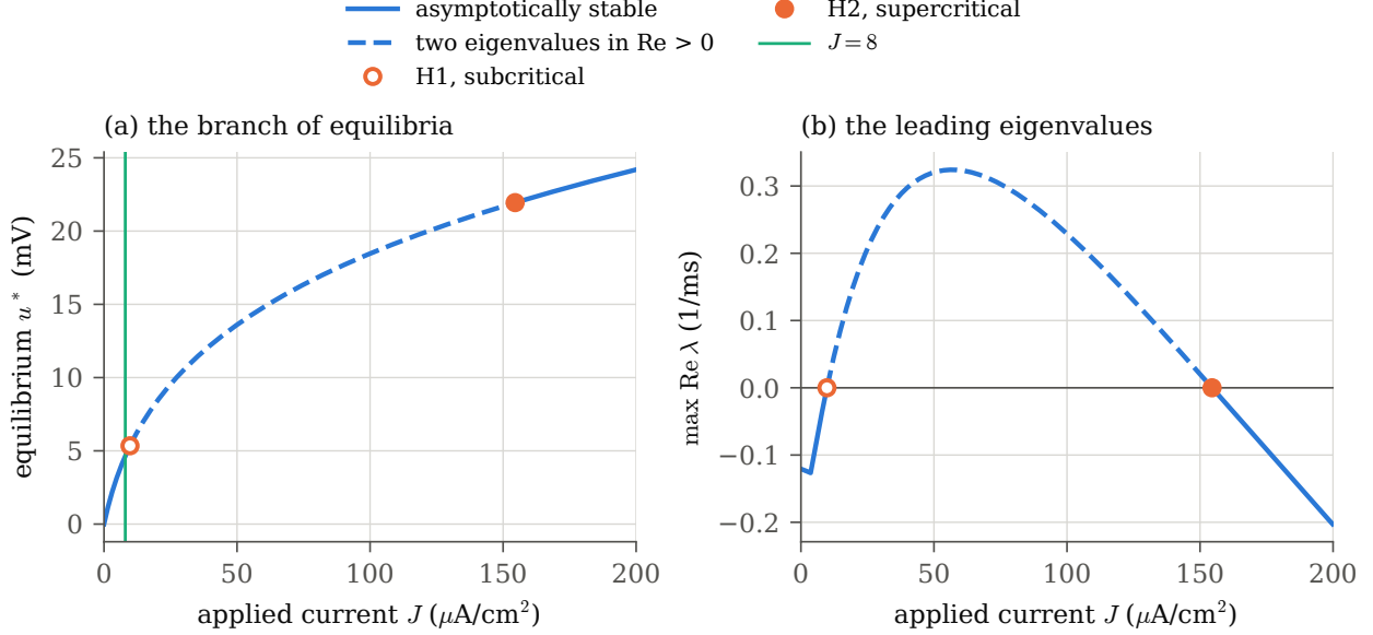
Figure 1: The branch of equilibria at E_l = 10.613 (code/hh_make_figures.py). (a) u^*(J) for J \in [0, 200] , solid where the equilibrium is asymptotically stable and dashed where it has two eigenvalues with positive real part; circles: the Hopf points of Theorem 2; the vertical line is J = 8 , the current of Theorems 4 and 5. (b) The largest real part of an eigenvalue. The curves are floating-point evaluations; the positions of the Hopf points and the stability types are those proved in Theorem 2.
