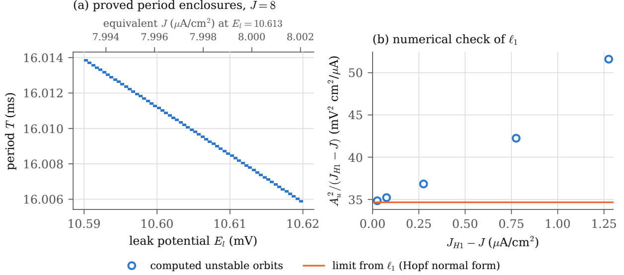
Figure 3: (a) Theorem 4: the proved enclosures of the period of \Gamma(E_l) on each of the 60 pieces of the E_l interval; the top axis gives the equivalent current at E_l = 10.613 (Lemma 2.2). (b) Numerical: A_u^2 / (J_{H1} - J) , where A_u is the peak-to-peak amplitude of u in mV, for the unstable periodic orbits computed in floating point at J = 8.5 to 9.75 ( E_l = 10.613 ; Table 5), and its limit 16|q_u|^2 \operatorname{Re} \lambda'(J_{H1}) / (\omega_1 \ell_1) \in [34.657379, 34.657380] predicted by the Hopf normal form from the proved values of Theorem 2 (Section 8).
