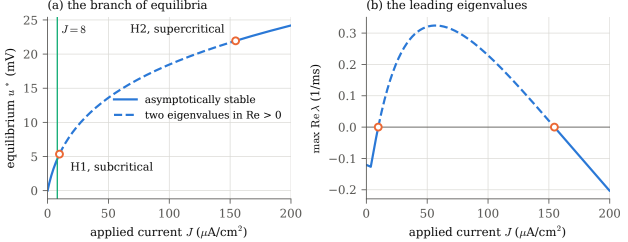
Figure 1: The branch of equilibria at E_l = 10.613 (code/hh_make_figures.py). (a) u^*(J) for J \in [0, 200] , solid where the equilibrium is asymptotically stable and dashed where it has two eigenvalues with positive real part; circles: the Hopf points of Theorem 2; the vertical line is J = 8 , the current of Theorems 4 and 5. (b) The largest real part of an eigenvalue. The curves are floating-point evaluations; the positions of the Hopf points and the stability types are those proved in Theorem 2.
