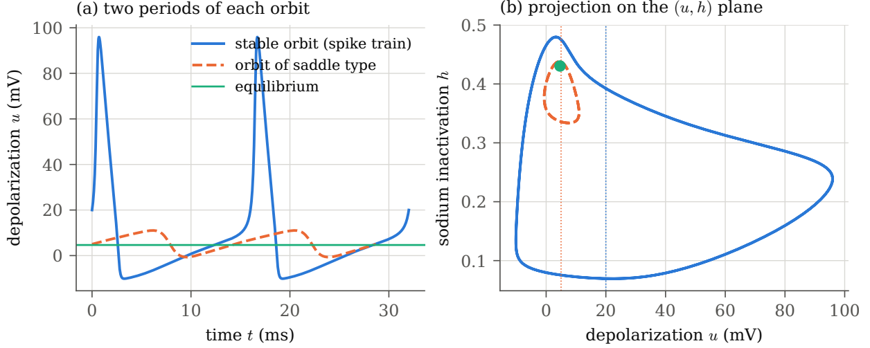
Figure 2: The orbits of Theorem 5 at J = 8 , E_l = 10.613 , integrated in floating point from the high-precision section points of Section 8 ( code/hh_make_figures.py ). (a) u(t) over two periods of the stable orbit \Gamma_s (solid) and of the saddle-type orbit \Gamma_u (dashed), and the equilibrium u^* . (b) The projection on the (u, h) plane, with the sections u = 20 and u = 5 (dotted) and the equilibrium (dot). The enclosures of the theorems are far narrower than the lines.
