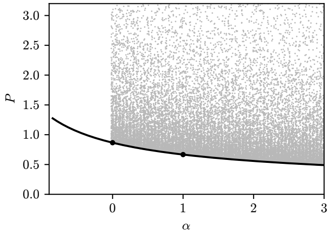
(a) P > \sqrt{3 + \alpha} / (2 + \alpha)
