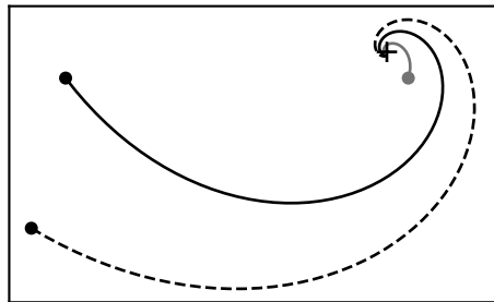
(b) SQG collapse, P = 0.788
