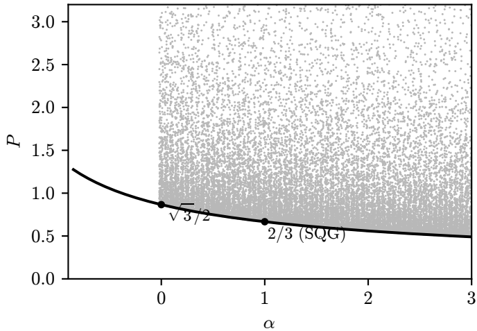
(a) P > \sqrt{3 + \alpha} / (2 + \alpha)
