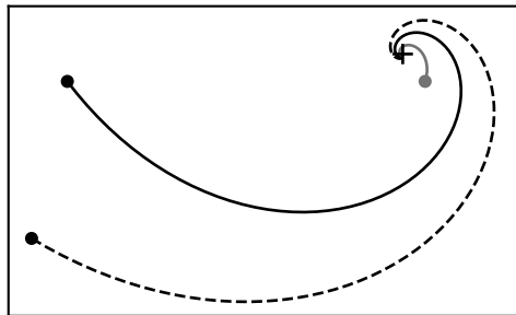
(b) SQG collapse, P = 0.788
