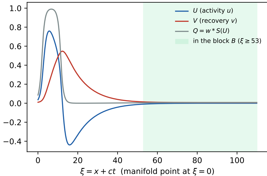
fast pulse, c = 1.10274770973\dots
