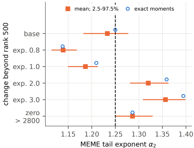
(b) MEME fits to 20 data sets
