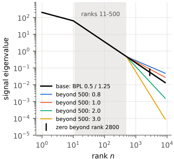
(a) Spectra sharing ranks 1-500
