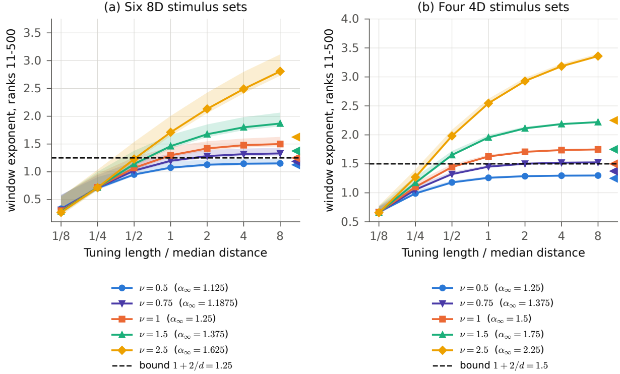
Figure 1: Ranks 11–500 window exponent of noise-free Matérn codes (infinitely many neurons) on the real stimulus coordinates, against the tuning length scale. Lines: median over the stimulus sets; bands: range over the sets. Arrowheads on the right: \alpha_\infty = 1 + 2\nu/d . Dashed line: the bound 1 + 2/d . Deterministic. Table 3 gives the effect of finite populations, the rank window, the metric and the number of stimuli.
