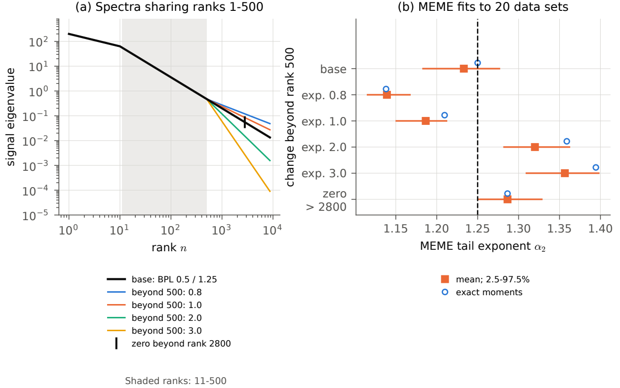
Figure 3: Left: the base spectrum, a broken power law with exponents 0.5 and 1.25, and variants that agree with it up to rank 500; shaded: ranks 11–500. Right: MEME \alpha_2 (diagonal weights) for each spectrum; squares and bars, mean and 2.5th–97.5th percentiles over 20 simulated data sets with common random numbers; circles, the fit to the exact moments. Dashed: the base tail exponent 1.25.
