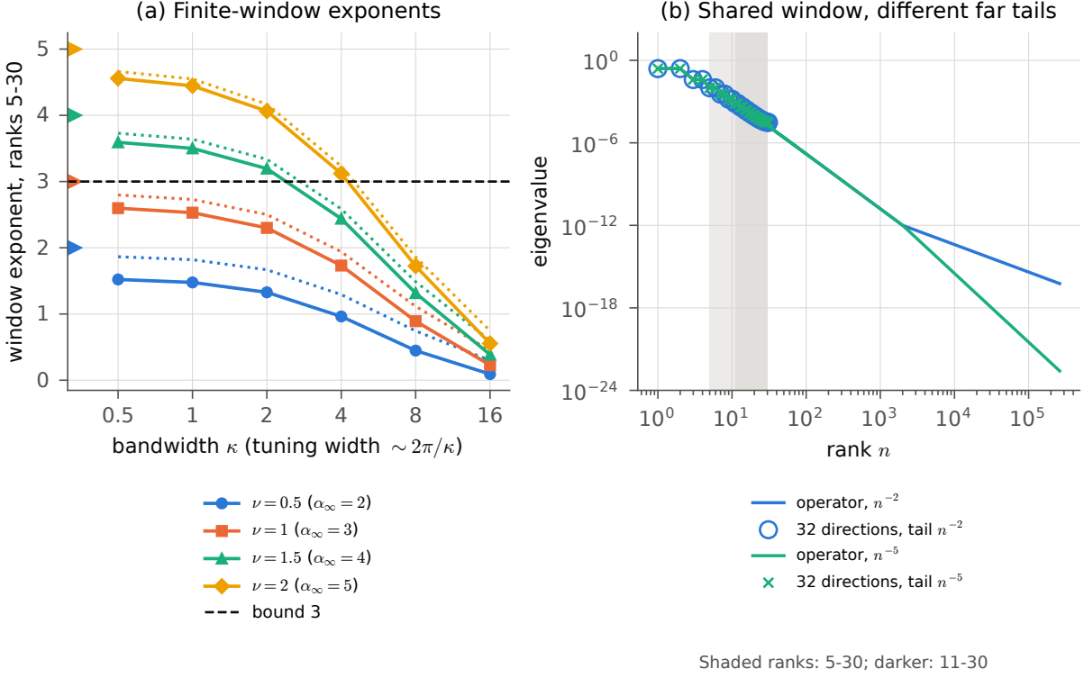
Figure 2: Left: ranks 5–30 window exponent (the window of the Methods of [1]; the text gives ranks 11–30, the window of their deposited code) for 32 equally spaced directions (solid) and for the operator spectrum without sampling (dotted), against the bandwidth \kappa of the tuning; arrowheads: \alpha_\infty = 1 + 2\nu ; dashed: the bound 3. Right: the numerical example of Proposition 1. Two codes share the differentiable \nu = 1.5 , \kappa = 1 spectrum up to frequency 1,000 and continue as n^{-2} (not differentiable) or n^{-5} (differentiable). Lines: operator spectra, with the far tails shown down to 10^{-24} ; markers: their 32-direction spectra, which are indistinguishable at this scale; both have window exponent 3.5012 over ranks 5–30 and 3.4306 over ranks 11–30, above the bound 3.
