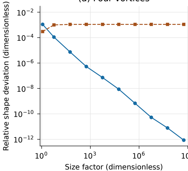
(a) Four vortices
