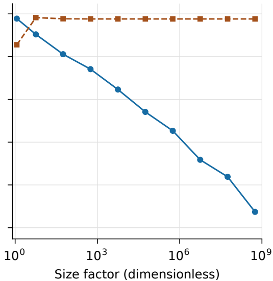
(b) Five vortices
