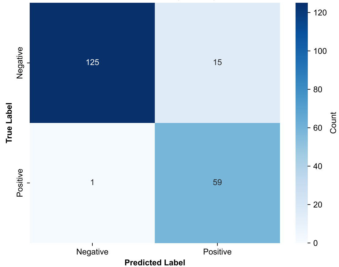
Confusion Matrix (Counts)
