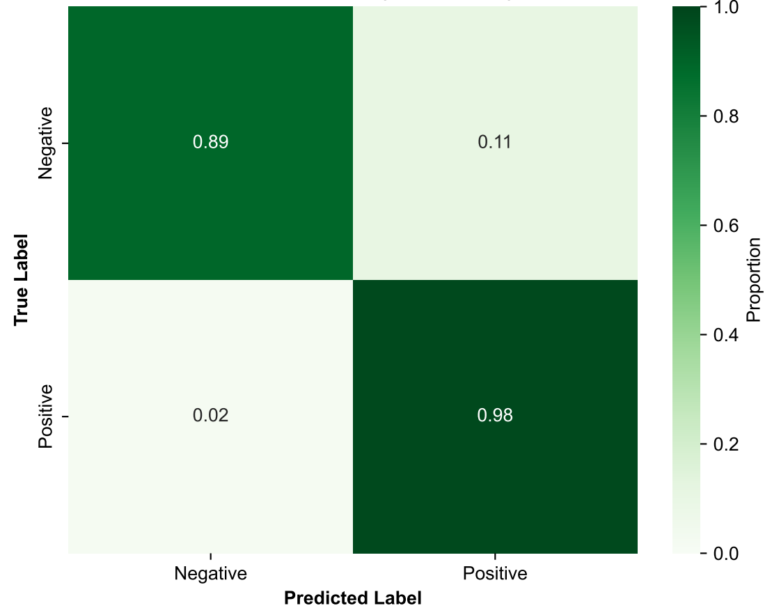
Confusion Matrix (Normalized)
