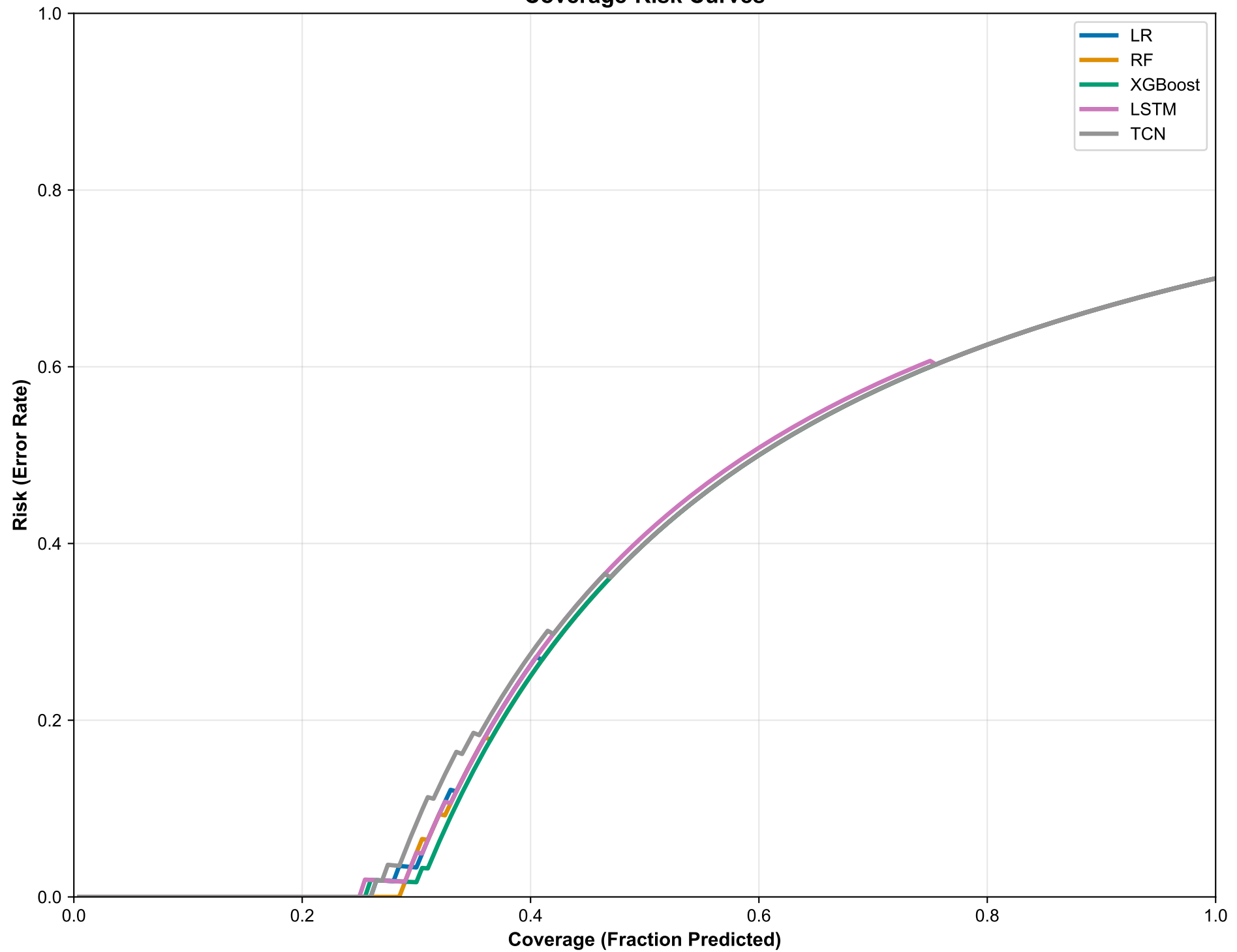
Coverage-Risk Curves
