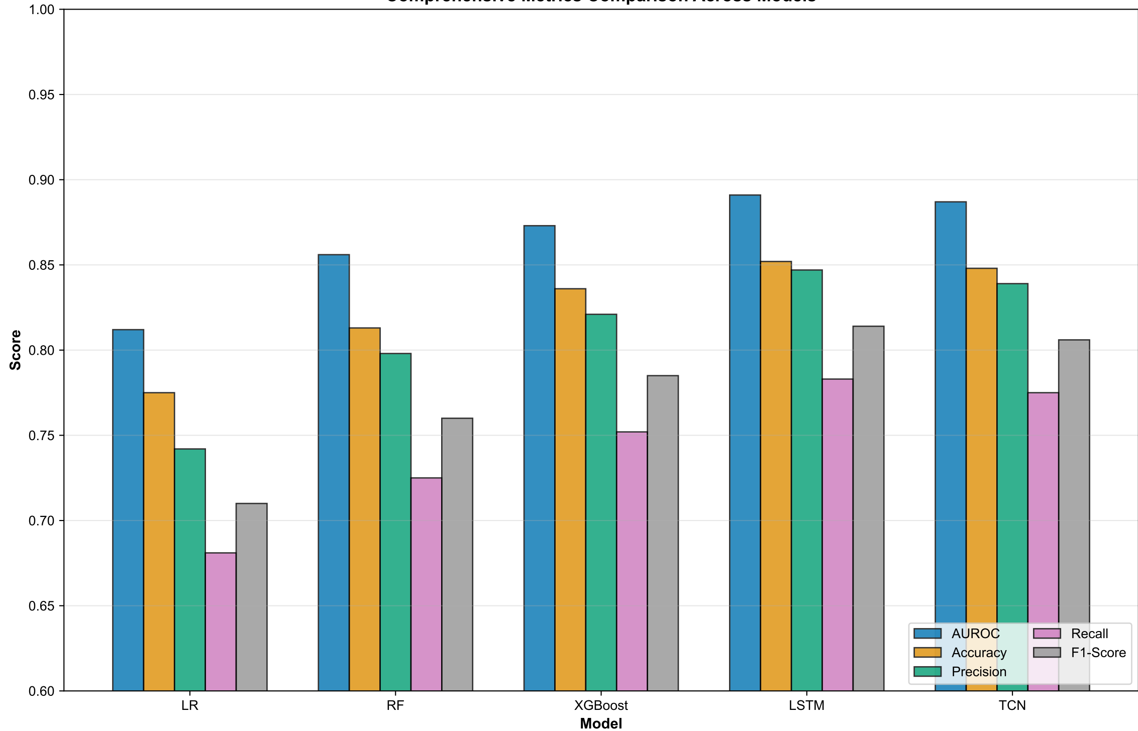
Comprehensive Metrics Comparison Across Models
