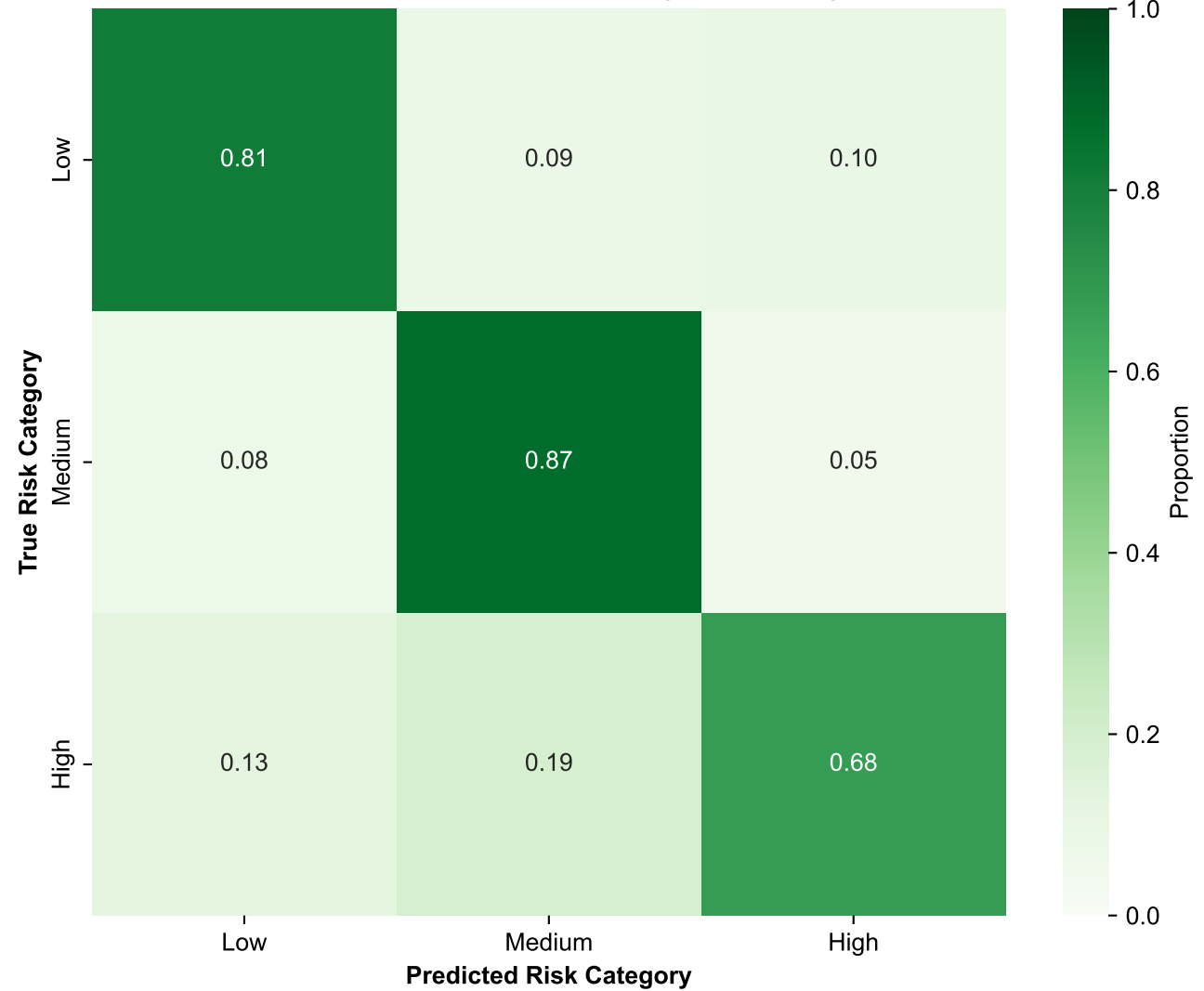
Multiclass Confusion Matrix (Normalized)
