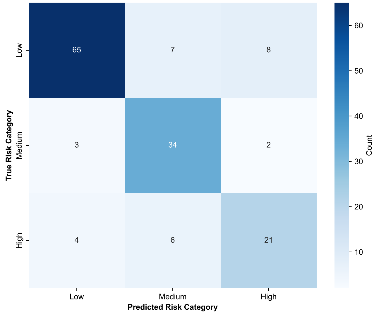
Multiclass Confusion Matrix (Counts)
