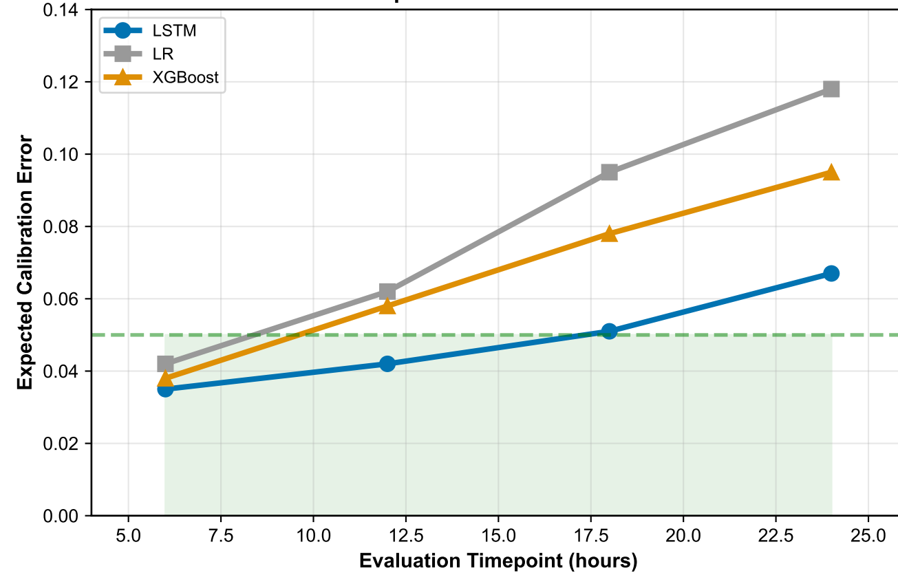
D. Temporal Calibration Evolution
