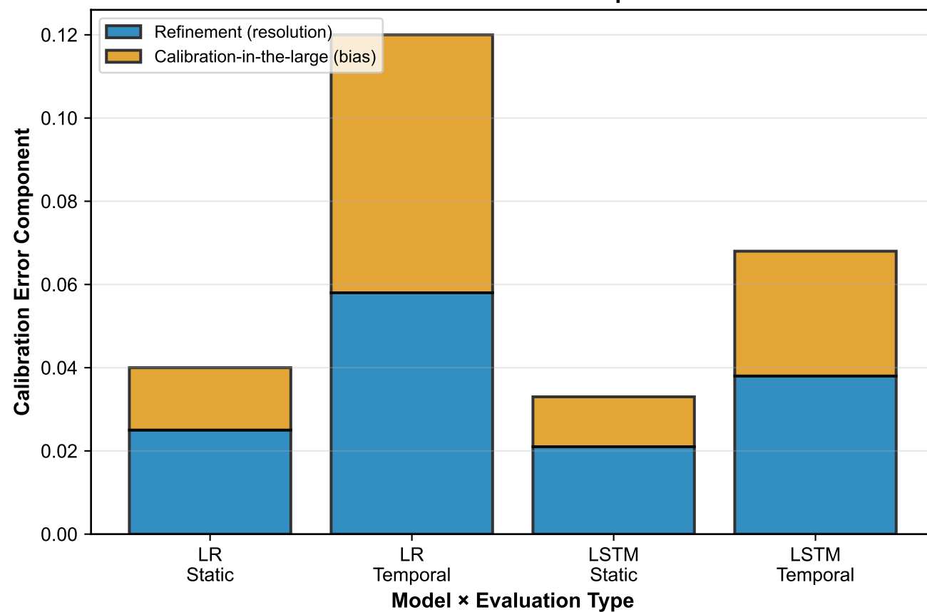
C. Calibration Error Decomposition
