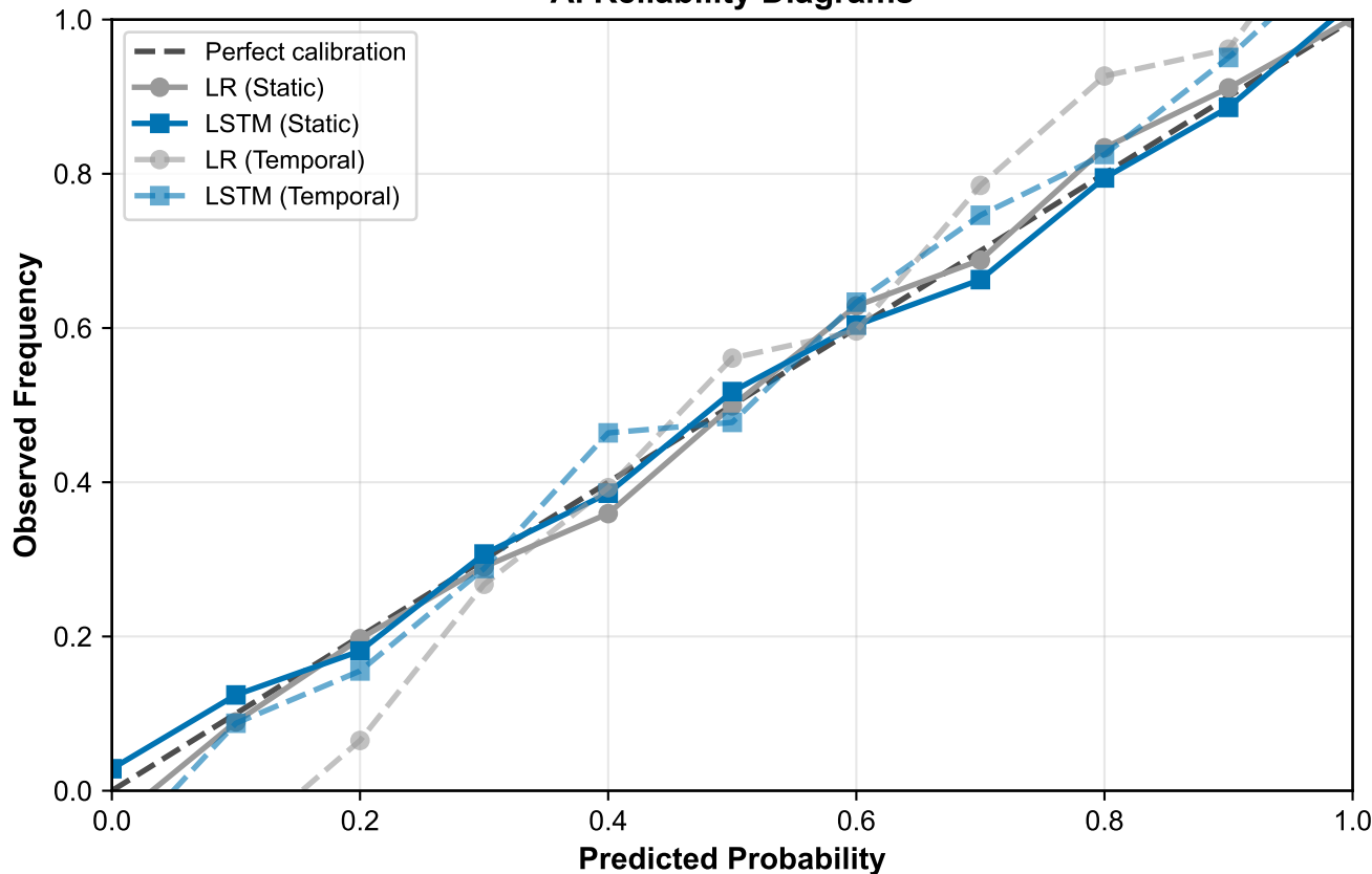
A. Reliability Diagrams
