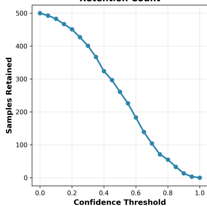
Retention Count
