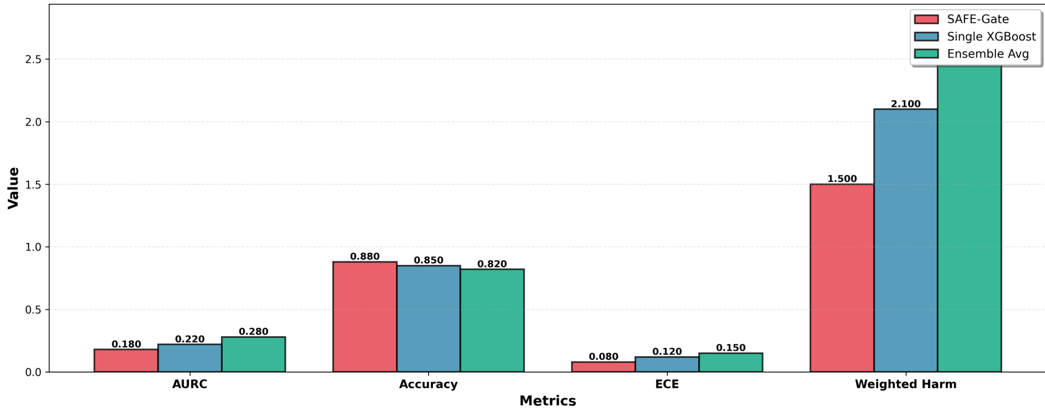
Multi-Model Performance Comparison
