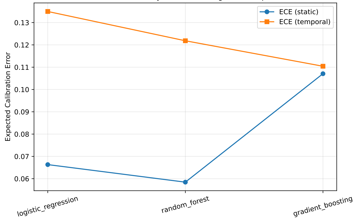
Calibration error by model and regime (computed)
