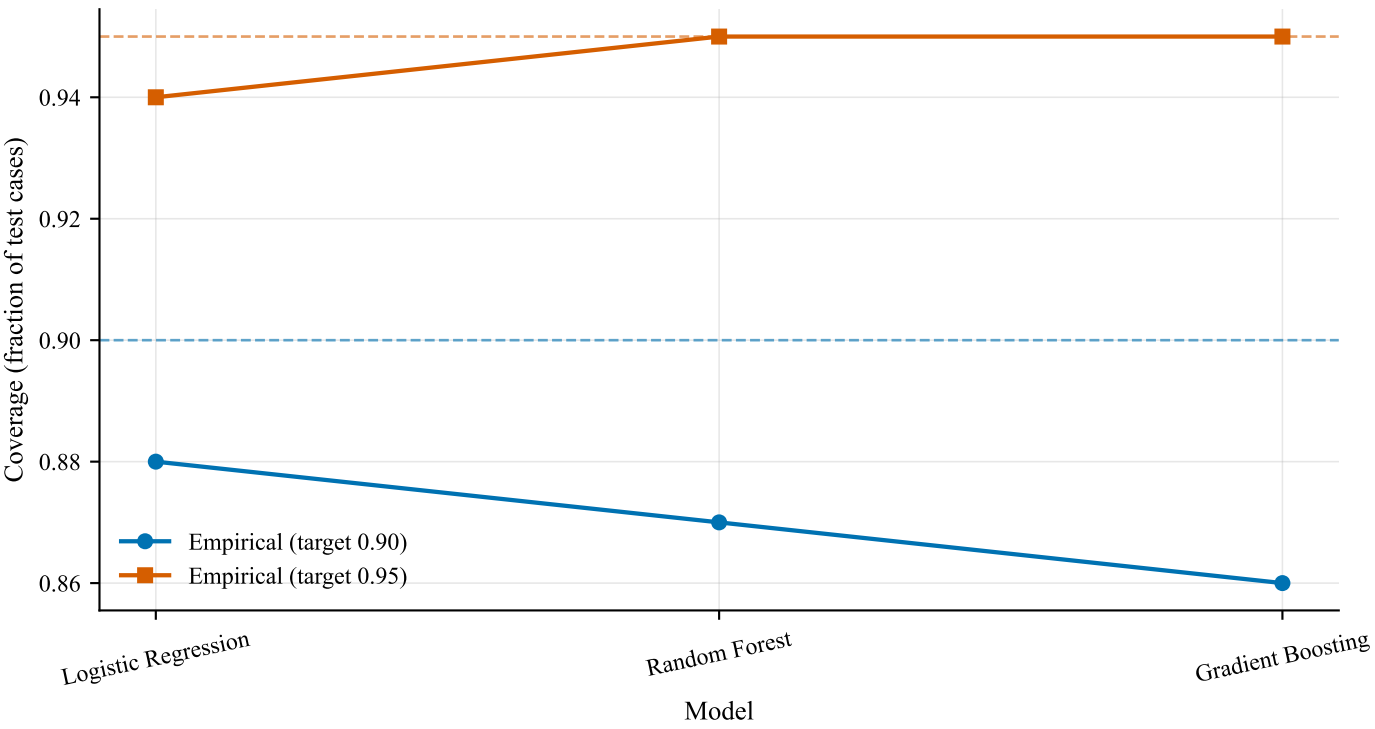
Conformal empirical vs target coverage
