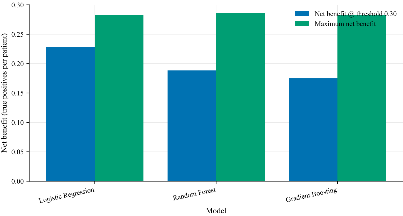
Decision-curve net benefit
