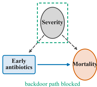
(B) Conditioning on Z = \{\text{Severity}\}
