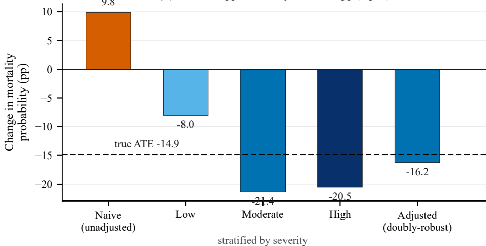
(C) Naive 9.8 pp versus adjusted -16.2 pp (sepsis)
