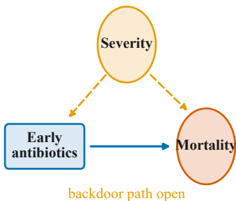
(A) Original DAG
