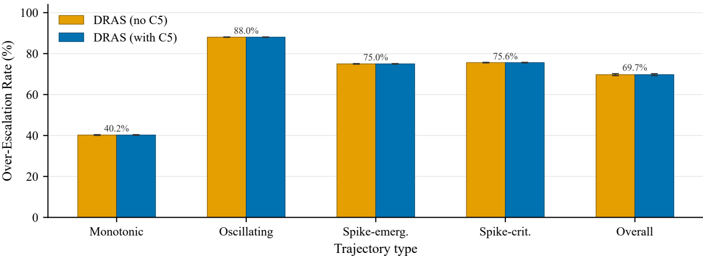
Over-Escalation Rate by Trajectory Type (seed 42; error bars = bootstrap 95% CI, N=1000); binary OER is near-identical with/without C5
