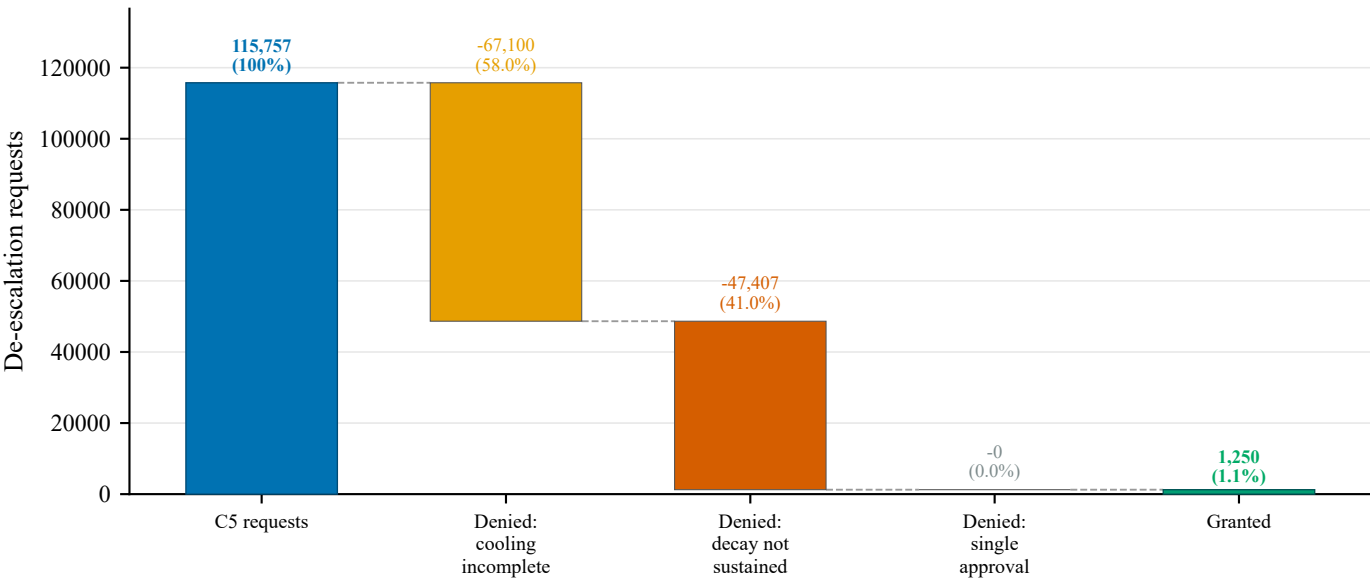
C5 De-escalation Outcome Funnel (n = 115,757, seed 42): 1,250 granted, each clearing the cooling/decay/dual-approval guards (0 premature)
