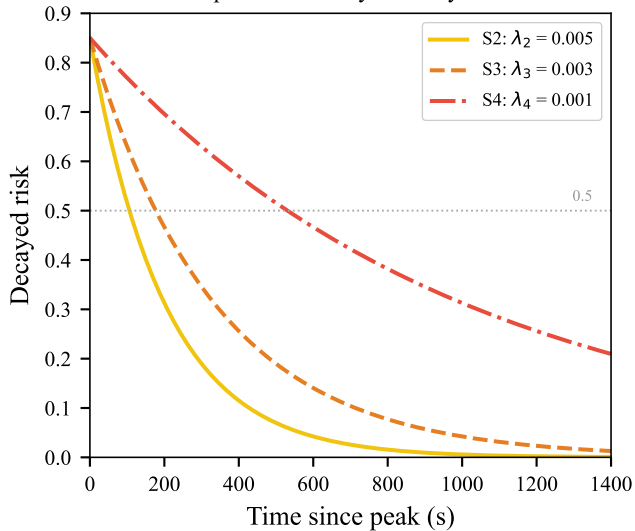
Exponential Decay Rates by State
