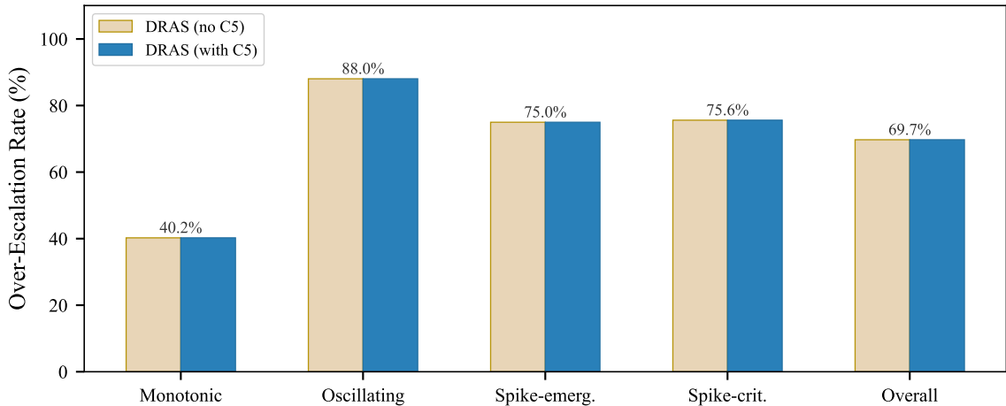
Over-Escalation Rate by Trajectory Type (seed 42); binary OER is near-identical with/without C5
