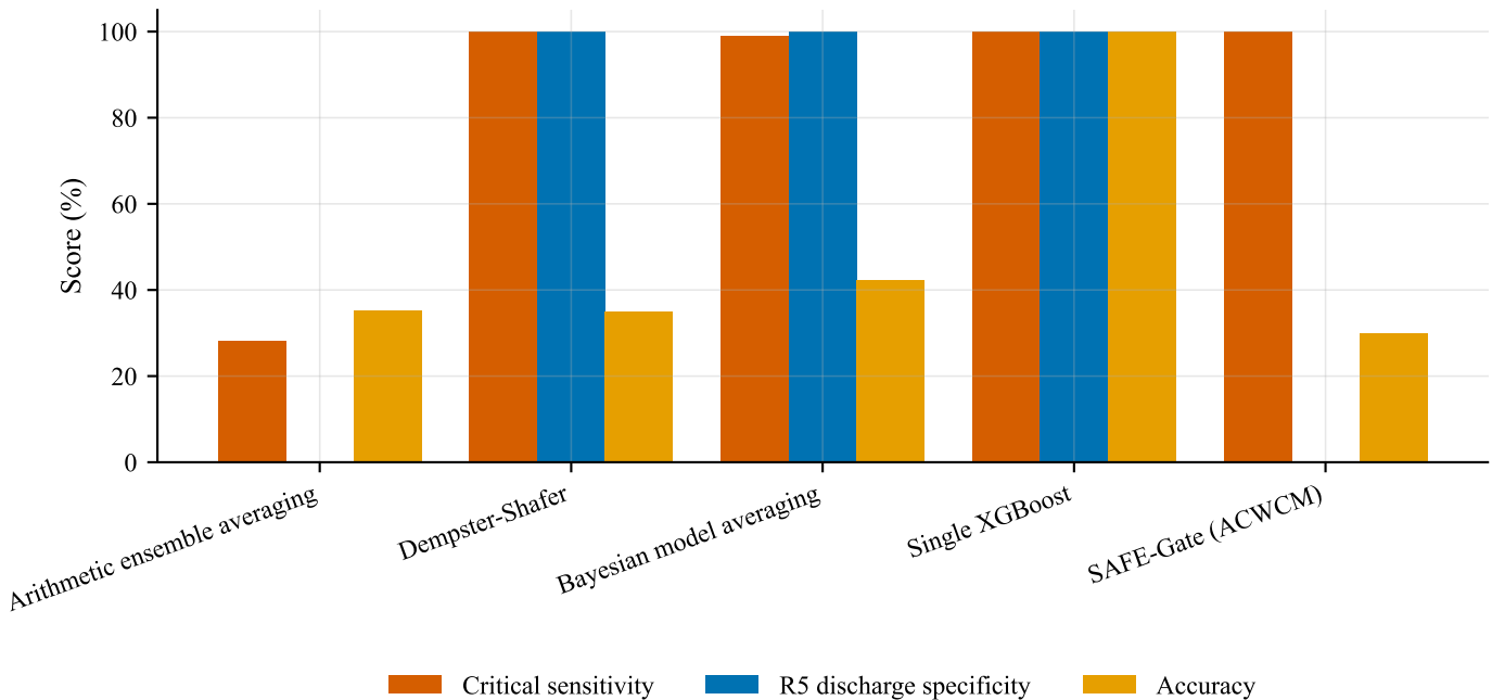
Baselines vs SAFE-Gate (test fold, seed 42)
