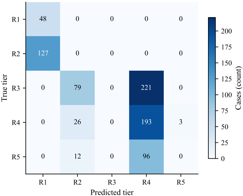
SAFE-Gate (ACWCM) confusion matrix (test fold, seed 42)
