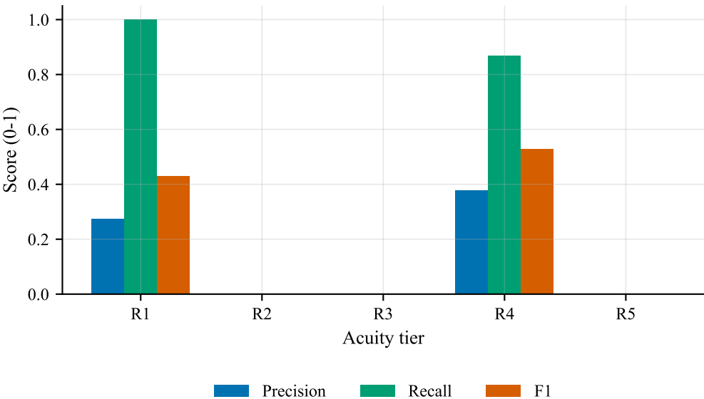
Per-tier classification metrics (test fold, seed 42)
