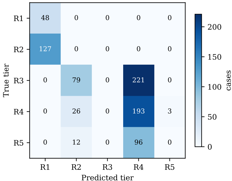
SAFE-Gate (ACWCM) confusion matrix (test fold, seed 42)
