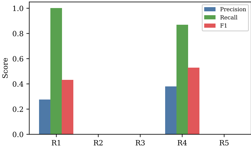
Per-tier metrics (test fold, seed 42)
