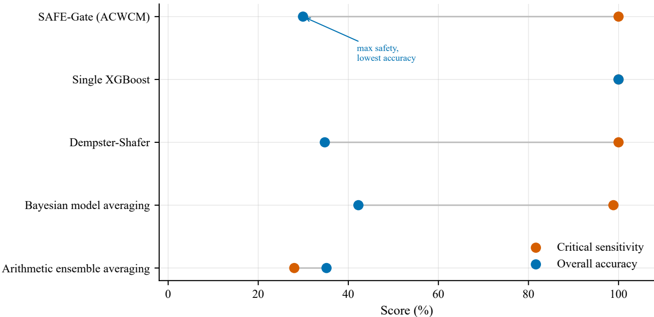
Safety vs accuracy trade-off across methods (test fold, seed 42)
