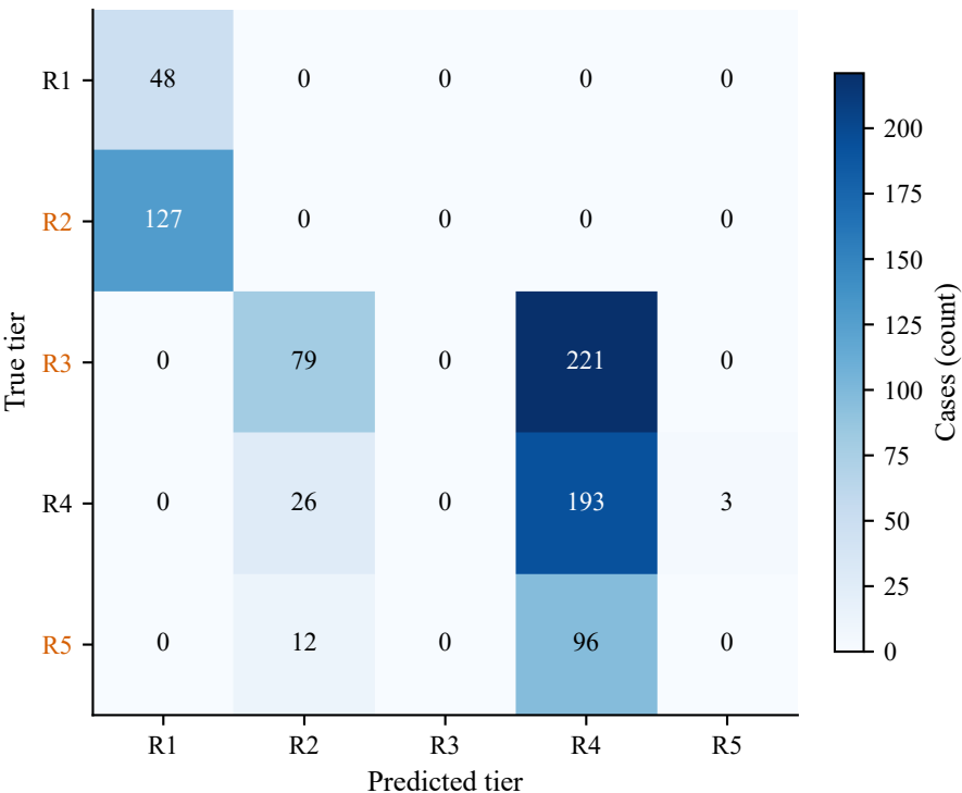
SAFE-Gate (ACWCM) confusion matrix (test fold, seed 42)
