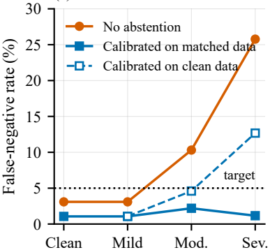
(a) FNR of decided cases
