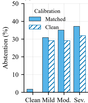
(b) Cases deferred
